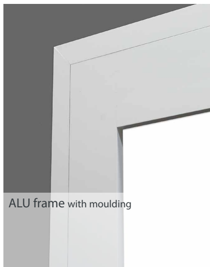
ALU frame (front installation) Lintel + frame legs Lintel 120 mm (suitable for LHR RM and R40) Lintel 180 mm (suitable for LHR FM) Frame legs 100 mm
