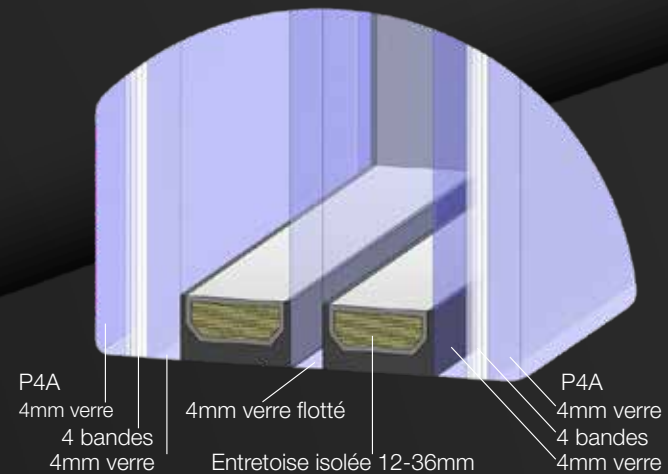
P4A + 4mm Float + P4A
