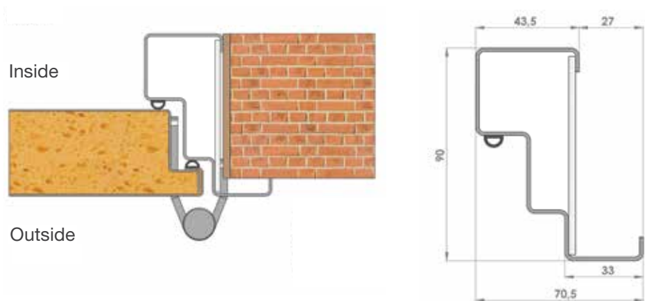
MITRED FRAME WITH MOULDINGS, OPEN TO OUTSIDE ( MO )
