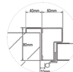
Frame dimensions
